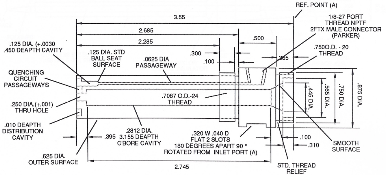
FIGURE 2-3: WATER INLET HOUSING
