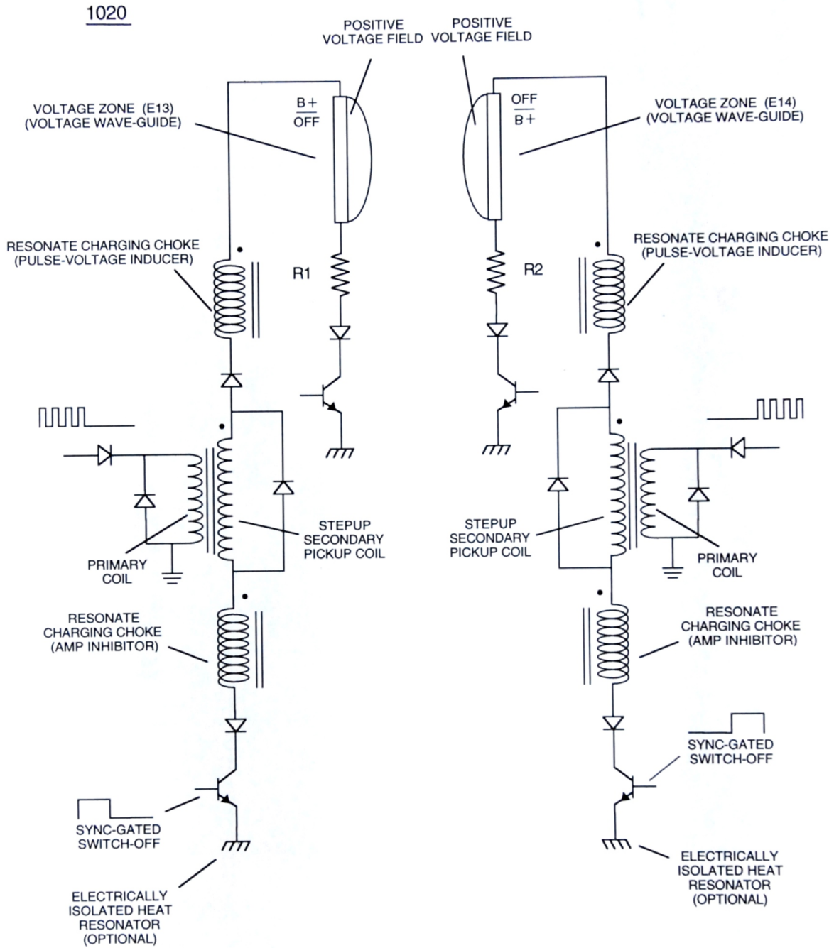
FIGURE 1-2: DUAL SWITCHOVER CIRCUIT
