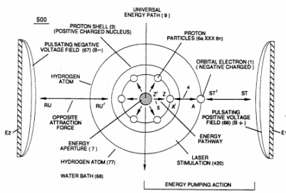
FIGURE 5-1: HYDROGEN ENERGY BALANCE
