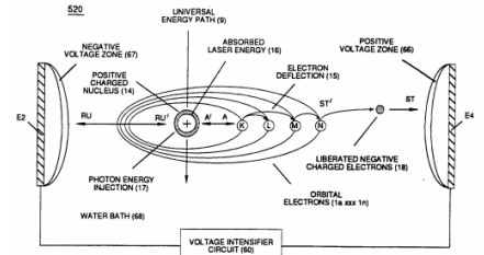
FIGURE 5-3: ENERGY PUMPING ACTION
