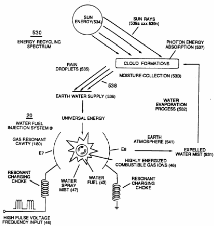
FIGURE 5-6: OPEN ENDED ENERGY SYSTEM
