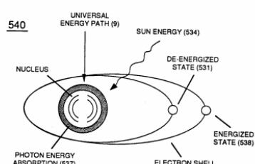
FIGURE 5-7: ATOMIC ENERGY LEVEL ADJUSTMENT
