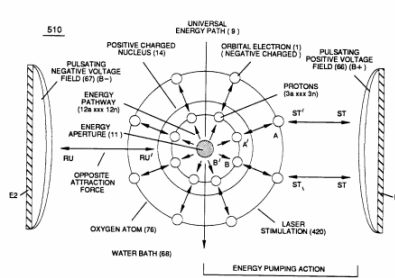
FIGURE 5-2: OXYGEN ENERGY BALANCE
