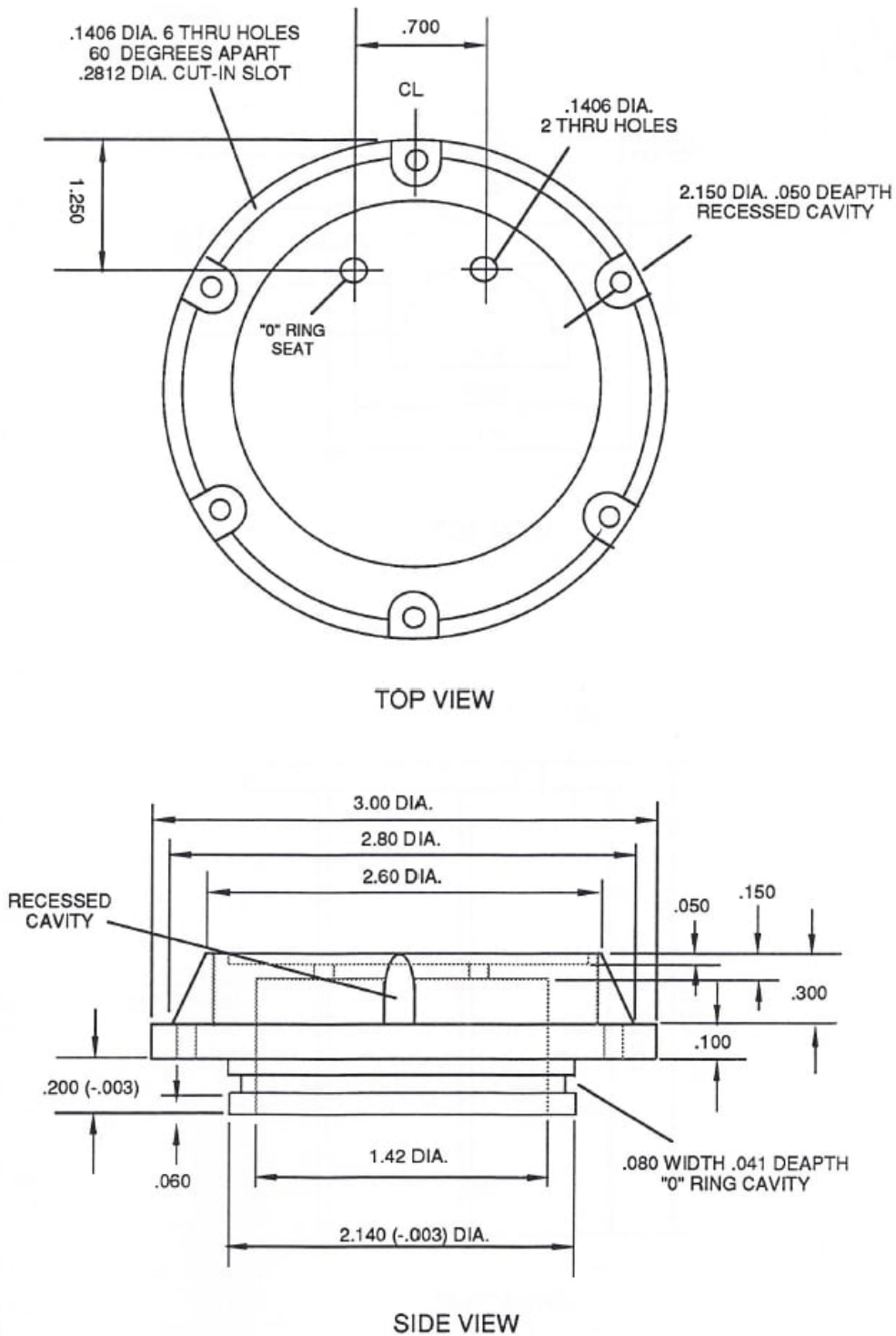
FIGURE 13-5: TERMINAL CAP
