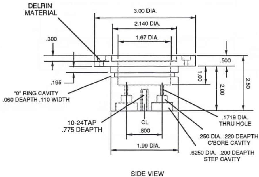
FIGURE 13-2: S/R MOUNT BASE
