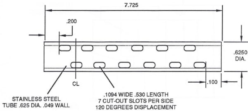
OUTER EXCITOR TUBE
