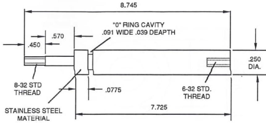
INNER EXCITOR ROD
