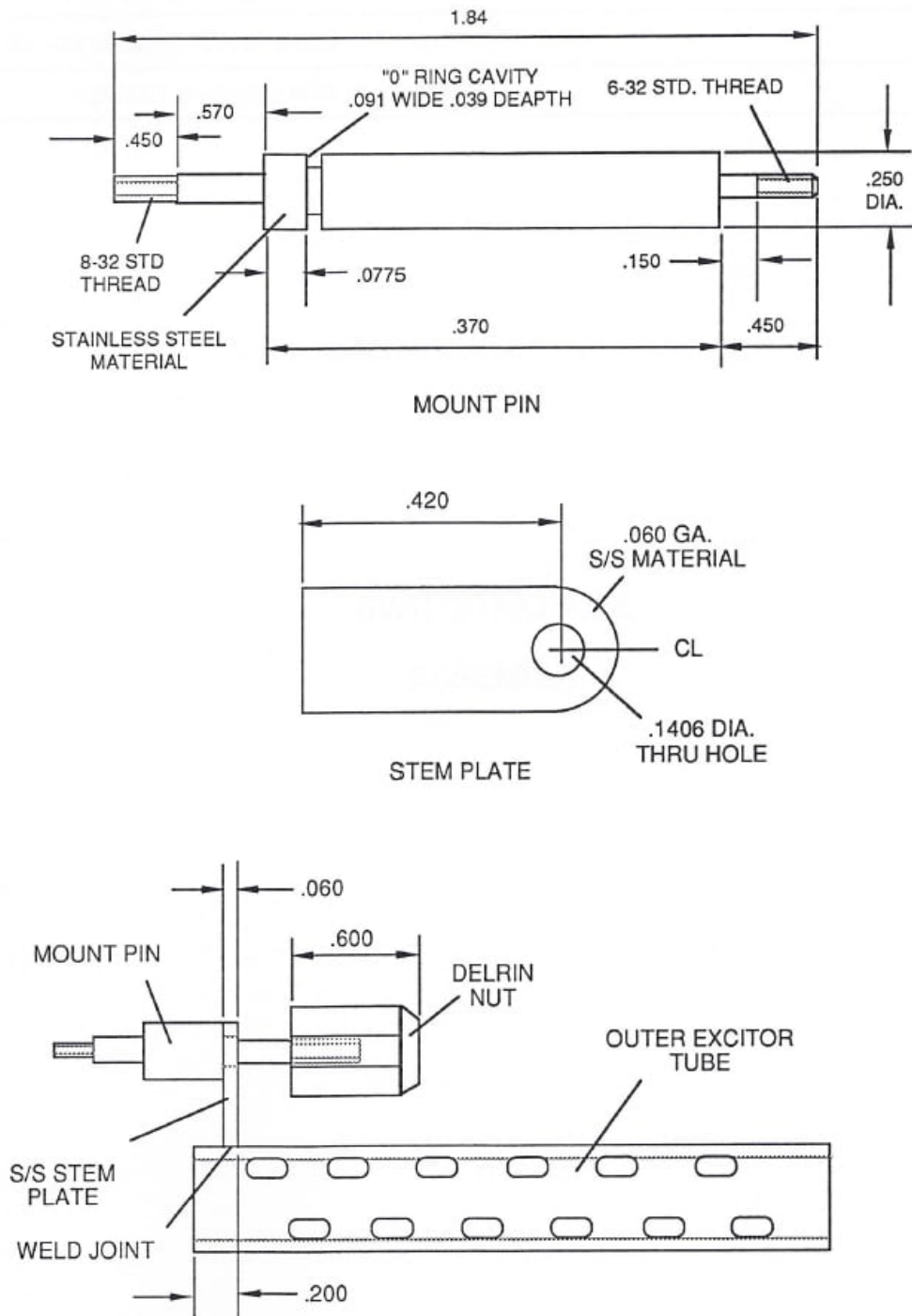
FIGURE 13-7: TERMINAL POST ASS'Y
