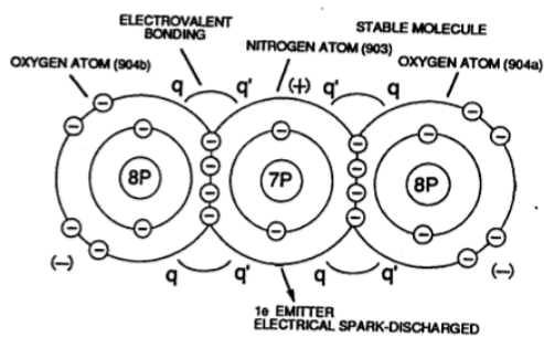
FIGURE 9-5: NITROGEN DIOXIDE NO 2
