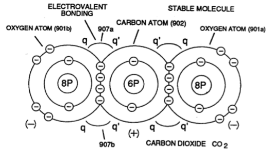
FIGURE 9-2: CARBON DIOXIDE CO 2
